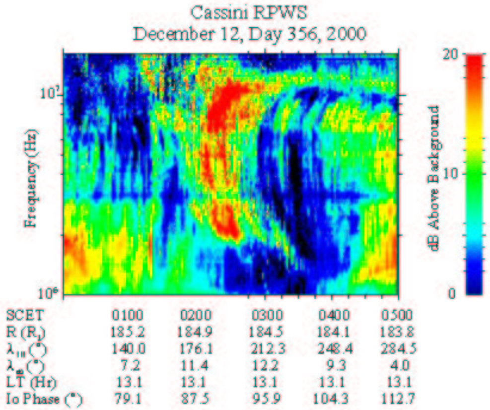
Figure 1: A time–frequency spectrogram showing the complicated arc structure associated with the DAM emission as observed by the Cassini spacecraft. The Io dependent enhancement of the emission from about 02:00 to 03:00 SCET ( \sim 87^\circ to \sim 96^\circ Io phase) is on the order of 20 dB more intense than the non–Io DAM emissions observed during this period.
